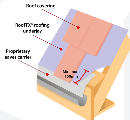
Figure 2 - Eaves Detail
