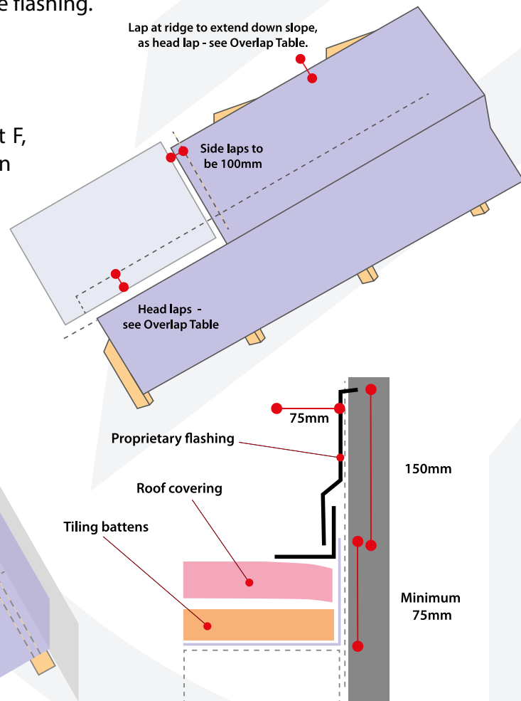
Figure 3 - Overlap Detail
